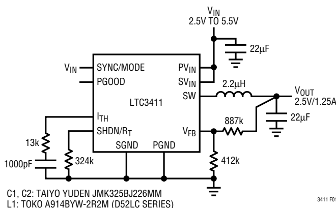
Figure 1. Step-Down 2.5V/1.25A Regulator
