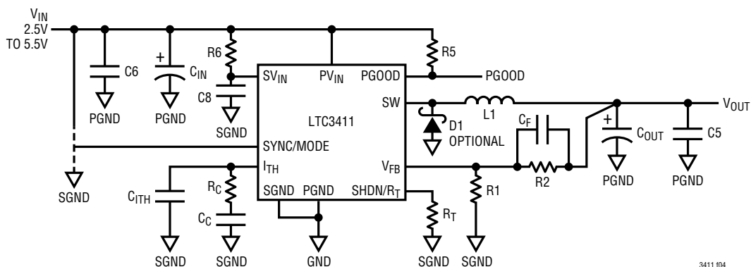
Figure 4. LTC3411 General Schematic
