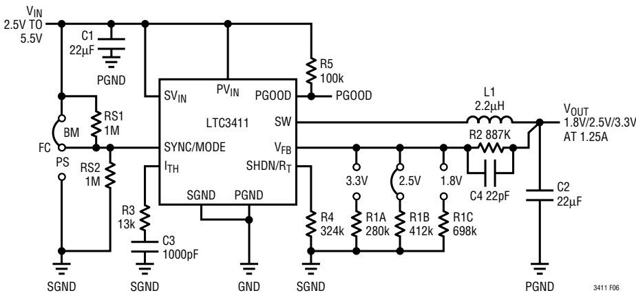
Figure 6. General Purpose Buck Regulator Using Ceramic Capacitors
