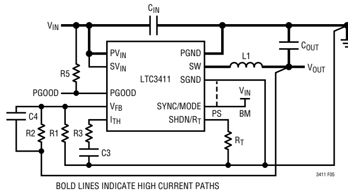
Figure 5. LTC3411 Layout Diagram (See Board Layout Checklist)
