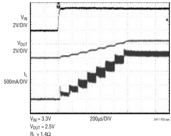
Figure 3. Digital Soft-Start
