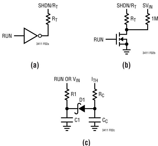
Figure 2. SHDN/R T Pin Interfacing and External Soft-Start
