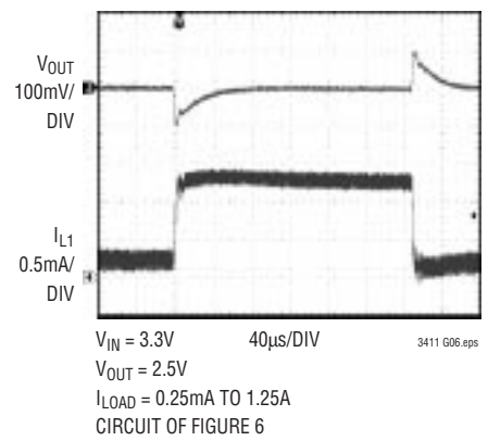
Load Step
